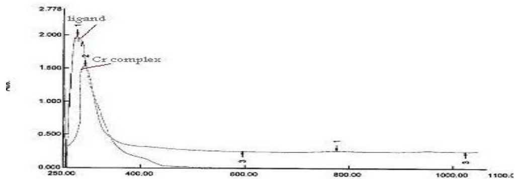
Figure 2: Electronic spectrum of the ligand and Cr - complexes.
