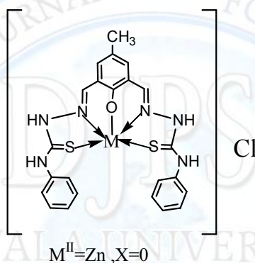
Scheme( 2): Proposed structures of complexes
