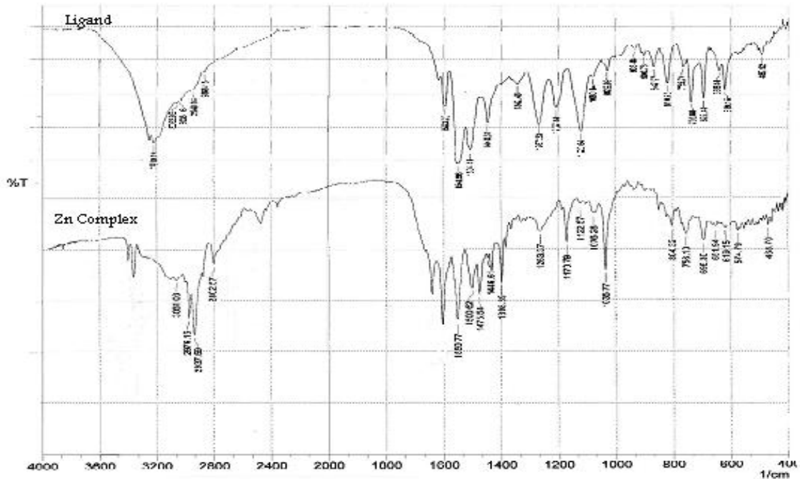
Figure 1: IR spectra for the ligand and Zn-complex
