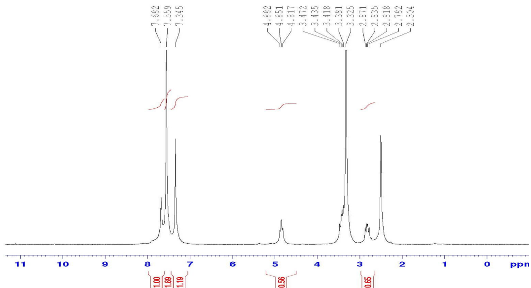
Figure 3: 1 H-NMR spectrum of the ligand HL in DMSO-d 6 solution.
